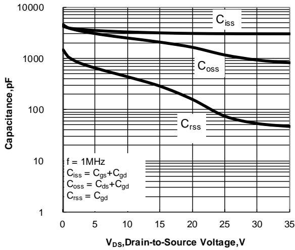
Figure 12. Capacitance Characteristics
