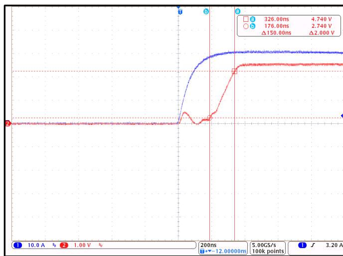
Figure 9. CT415 Rise Time; I P = 30 A PK and C L = 100 pF (Blue = I CC , Red = V OUT )
