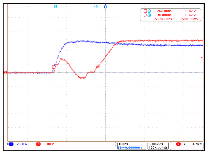
Figure 10. CT415 Propagation Delay; I P = 30 A PK and C L = 100 pF (Blue = I CC , Red = V OUT )
