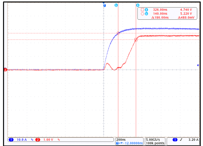
Figure 8. CT415 Response Time; I P = 30 A PK and C L = 100 pF (Blue = I CC , Red = V OUT )
