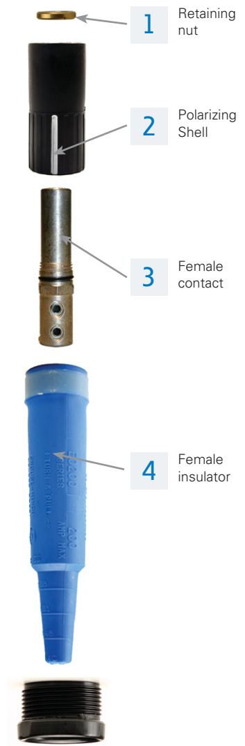
Female Plug Assembled length is 8 3/4"
