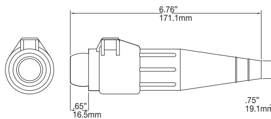
Female Connector
