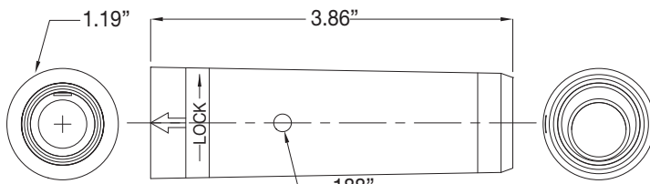
Male & Female Plug
