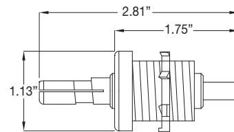
Male Receptacle
