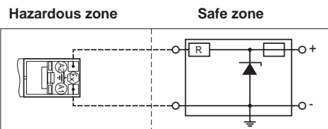
Sub-base for intrinsic safety miniature solenoid valve
