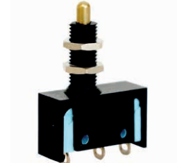
Telescopic plunger with 3 mm overtravel and with M6 x 0.75 threaded barrel
