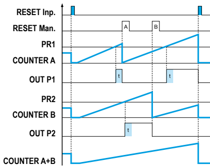
Output operation: OutoP MurS0 (AS)
