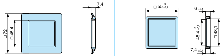
26546842 - Adaptor for 72 x 72 mm cut-out
