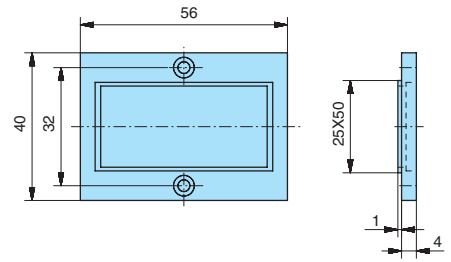
26546843 - Adaptor for 50 x 25 mm cut-out
