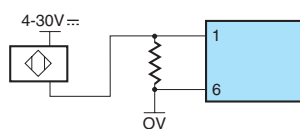
2-wire proximity sensor fast count input
