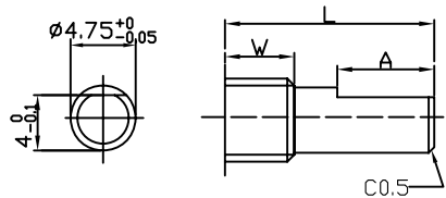
FE Shaft Style
