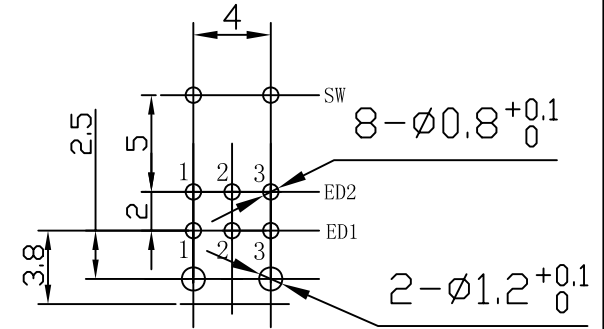
Mounting hole detail
