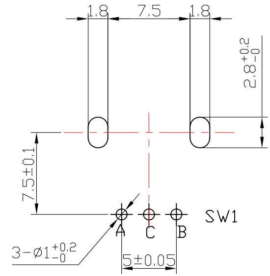
P. C. B MOUNTING DETAIL
