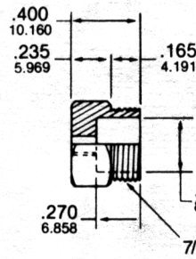
1/2" HEX BODY
