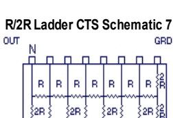
R/2R Ladder CTS Schematic 7
