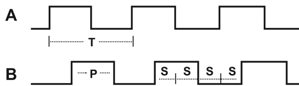
Figure 1 Quadrature signals showing counter-clockwise rotation
