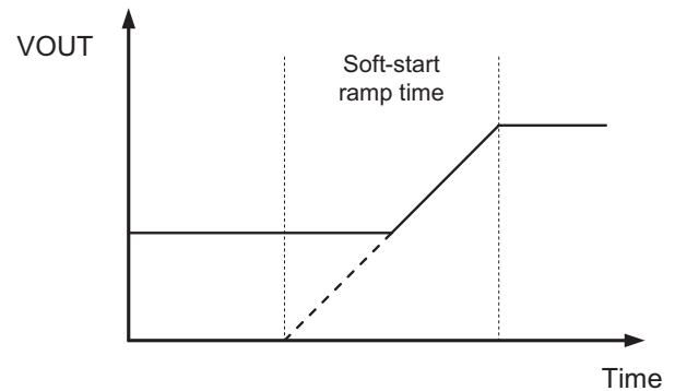
Illustration of Pre-Bias Startup.
