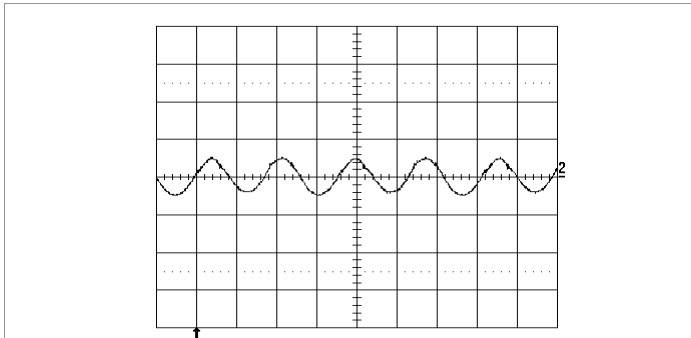
Output voltage ripple at: T_{P1}, T_{P3} = +25^{\circ}\text{C} , V_1 = 53\text{ V} , I_O = 39\text{ A} resistive load. Trace: output voltage (50 mV/div.). Time scale: (2 \mu\text{s} /div.).
