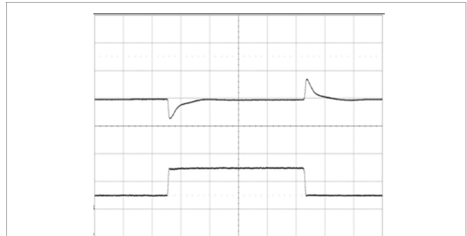
Output voltage response to load current step-change (9.75-29.25-9.75 A) at: T_{P1}, T_{P3} = +25^{\circ}\text{C} , V_1 = 53\text{ V} , C_O = 3.9\text{ mF} . Top trace: output voltage (0.5 V/div.). Bottom trace: output current (20 A/div.). Time scale: (0.5 ms/div.).
