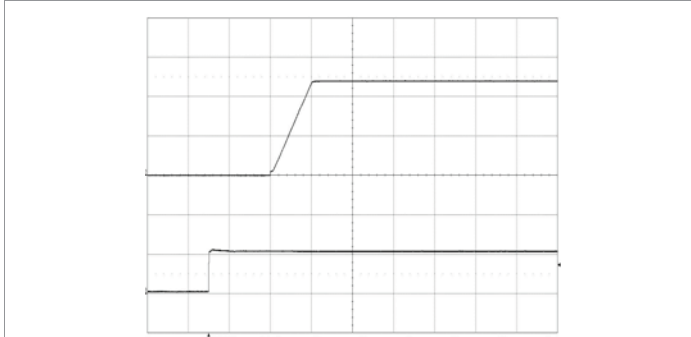
Start-up enabled by connecting V_1 at: T_{P1}, T_{P3} = +25^{\circ}\text{C} , V_1 = 53\text{ V} , I_O = 39\text{ A} resistive load. Top trace: output voltage (5 V/div.). Bottom trace: input voltage (50 V/div.). Time scale: (10 ms/div.).
