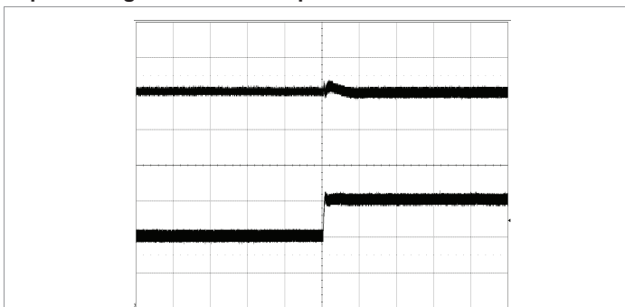
Output voltage response to input voltage transient at: T_{P1}, T_{P3} = +25^{\circ}\text{C} , V_1 = 40\text{-}60\text{ V} , I_O = 19.5\text{ A} resistive load, C_O = 3.9\text{ mF} . Top trace: output voltage (2 V/div.). Bottom trace: input voltage (20 V/div.). Time scale: (0.5 ms/div.).
