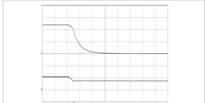
Shut-down enabled by disconnecting V_1 at: T_{P1}, T_{P3} = +25^{\circ}\text{C} , V_1 = 53\text{ V} , I_O = 39\text{ A} resistive load. Top trace: output voltage (5 V/div.). Bottom trace: input voltage (50 V/div.). Time scale: (2 ms/div.).
