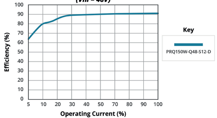
EFFICIENCY VS OUTPUT LOAD (Vin = 48V)
