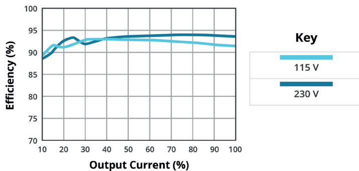
EFFICIENCY VS OUTPUT LOAD (VGS-500B-18)
