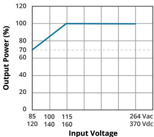
INPUT VOLTAGE DERATING CURVE (25°C)
