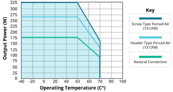
TEMPERATURE DERATING CURVE (15 Vdc output models)
