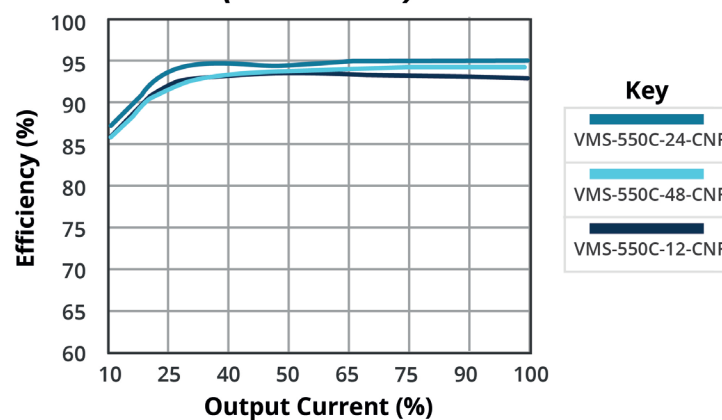
EFFICIENCY VS OUTPUT LOAD ( V_{in} = 230 \text{ Vac} )
