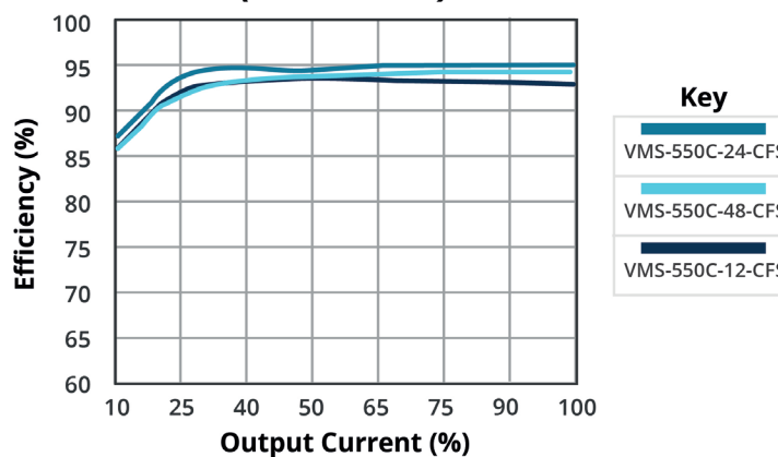
EFFICIENCY VS OUTPUT LOAD ( V_{in} = 230 \text{ Vac} )
