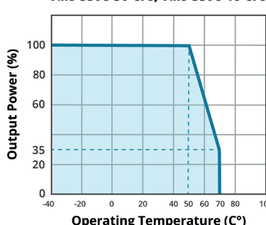
TEMPERATURE DERATING CURVE (full load 550W with 25 CFM) VMS-550C-24-CFS, VMS-550C-27-CFS VMS-550C-36-CFS, VMS-550C-48-CFS
