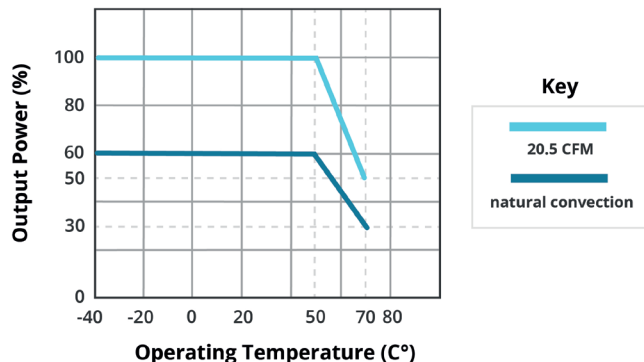
TEMPERATURE DERATING CURVE (full load 300W with 20.5 CFM) VOF-350C-12
