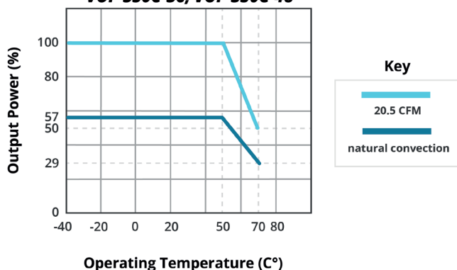
TEMPERATURE DERATING CURVE (full load 350W with 20.5 CFM) VOF-350C-24, VOF-350C-27 VOF-350C-36, VOF-350C-48
