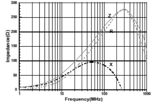
CMBH3216S181QSP
