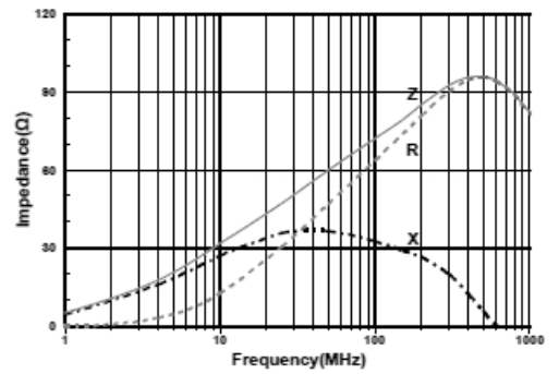
CMBH3216S750RSP
