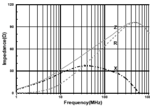
CMBH3216S900QSP
