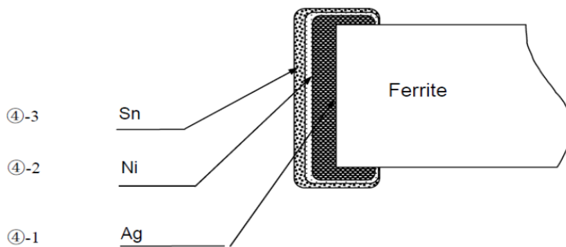
Fig.2 Body Structure
