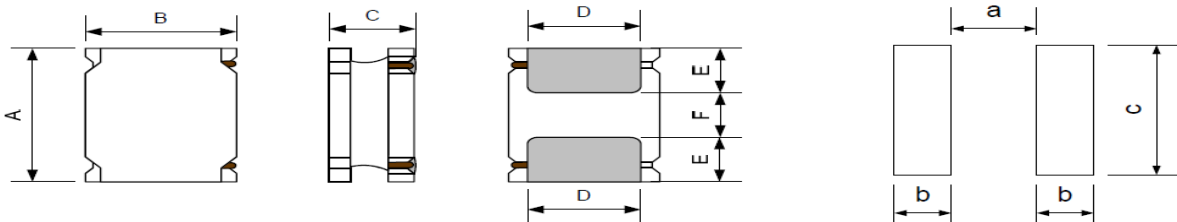
Recommended Land Pattern
