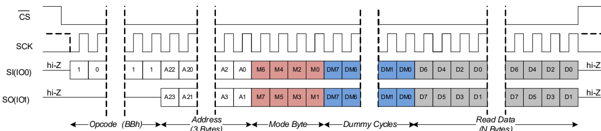
Figure 60. Double I/O Read (DIOR)
