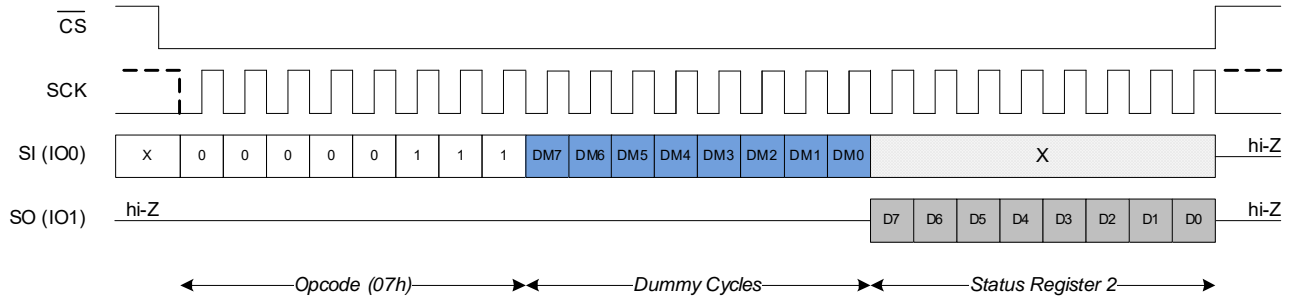
Figure 18. Read SR2 (RDSR2) in SPI Mode
