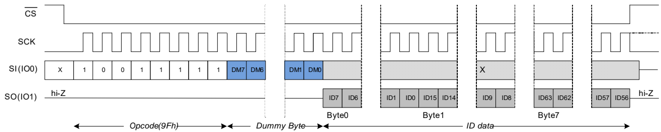
Figure 87. Read Device ID (RDID) in SPI Mode
