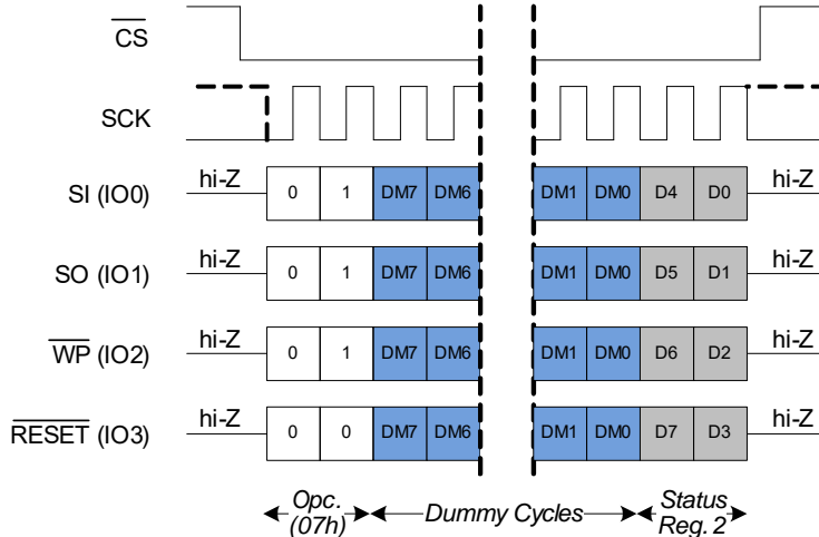
Figure 20. Read SR2 (RDSR2) in QPI Mode
