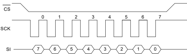
Figure 5. SPI Mode 3
