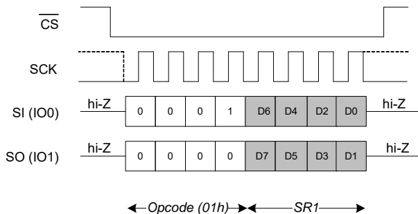
Figure 13. WRSR in DPI Mode (WREN not shown)
