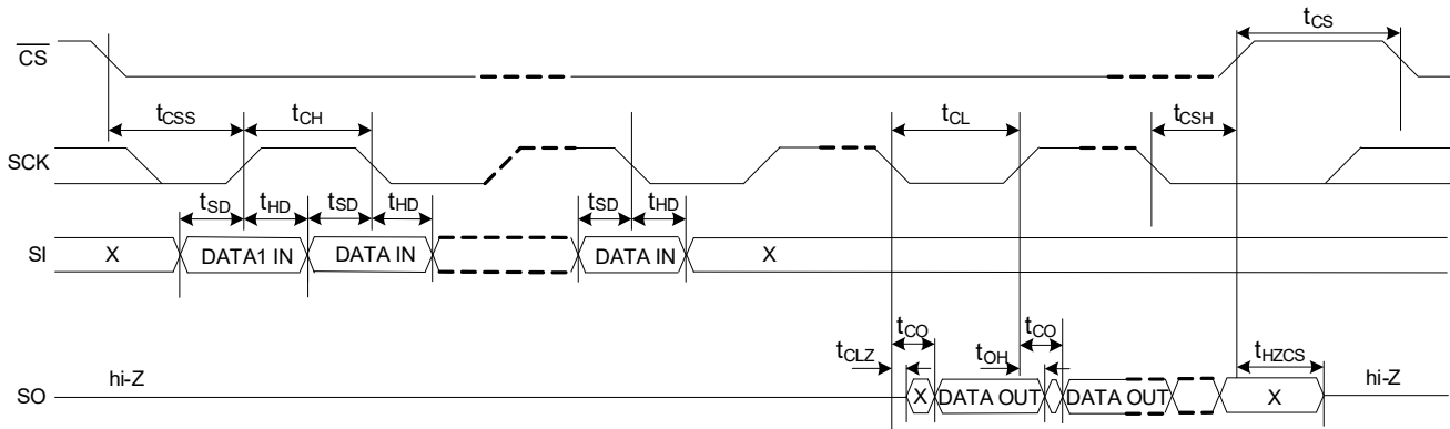
Figure 117. SPI Switching Timing - Single I/O, DDR
