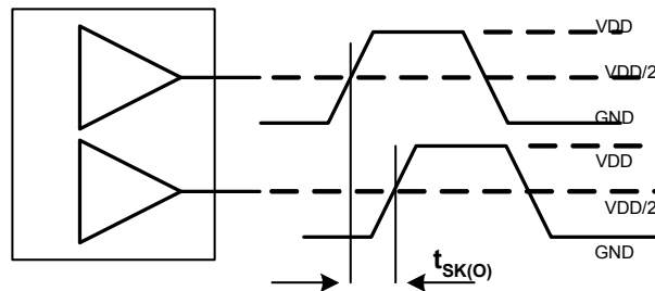
Figure 4. Output-to-Output Skew, t_{sk(O)}
