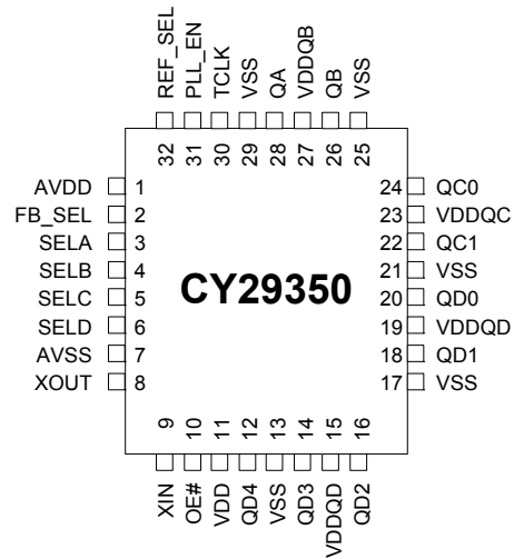
Figure 1. 32-pin TQFP pinout
