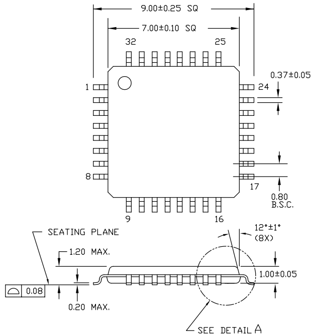
Figure 5. 32-pin TQFP (7 × 7 × 1.0 mm) Package Outline, 51-85063
