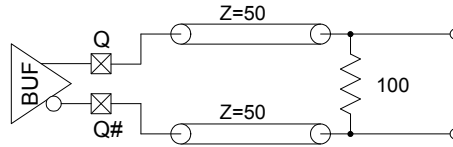
Figure 3. Input Differential and Common Mode Voltages
