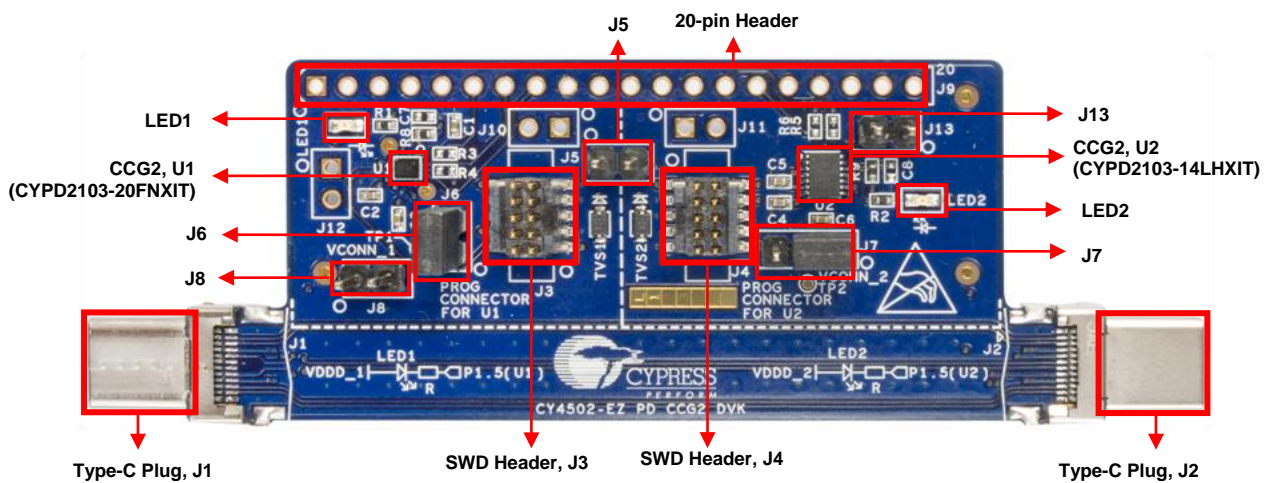
Figure 4-2. CY4502 Board
