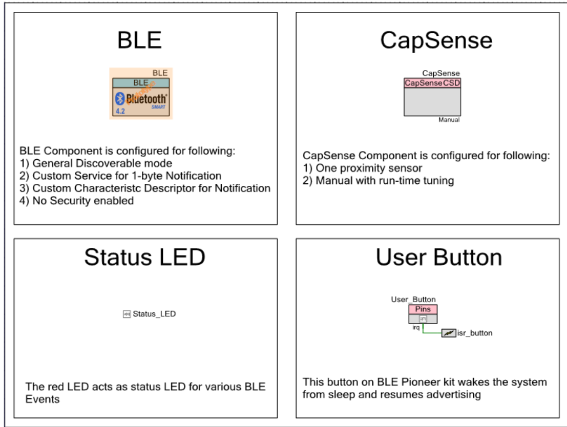
Figure 4-31. Top Design for PProC_BLE_CapSense_Proximity Project
