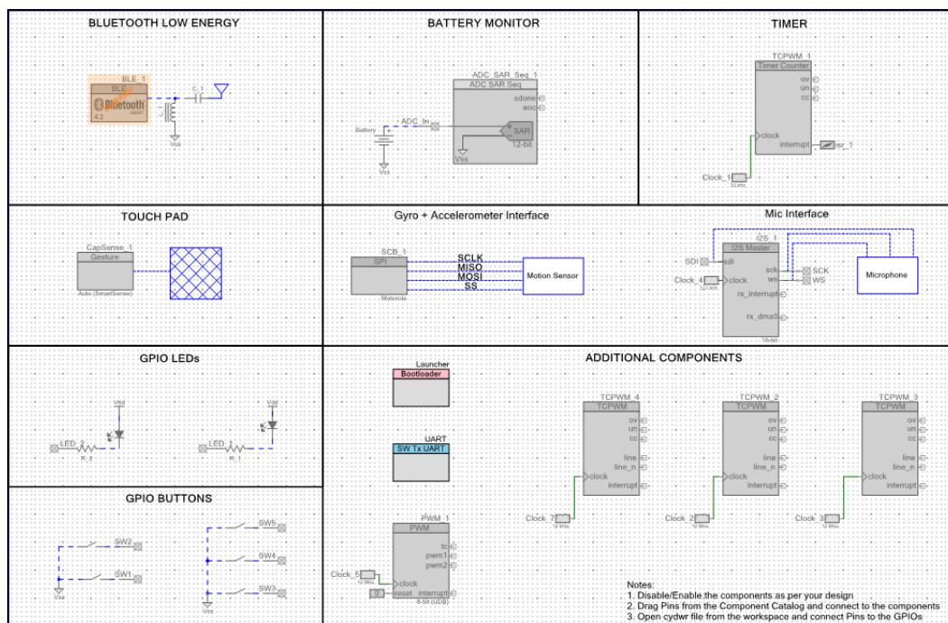
Figure 4-77. TopDesign for PSoC_BLE_OTA_Launcher Project
