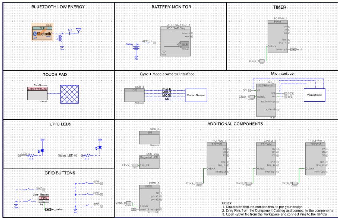
Figure 4-31. Top Design for PProC_BLE_CapSense_Proximity Project
