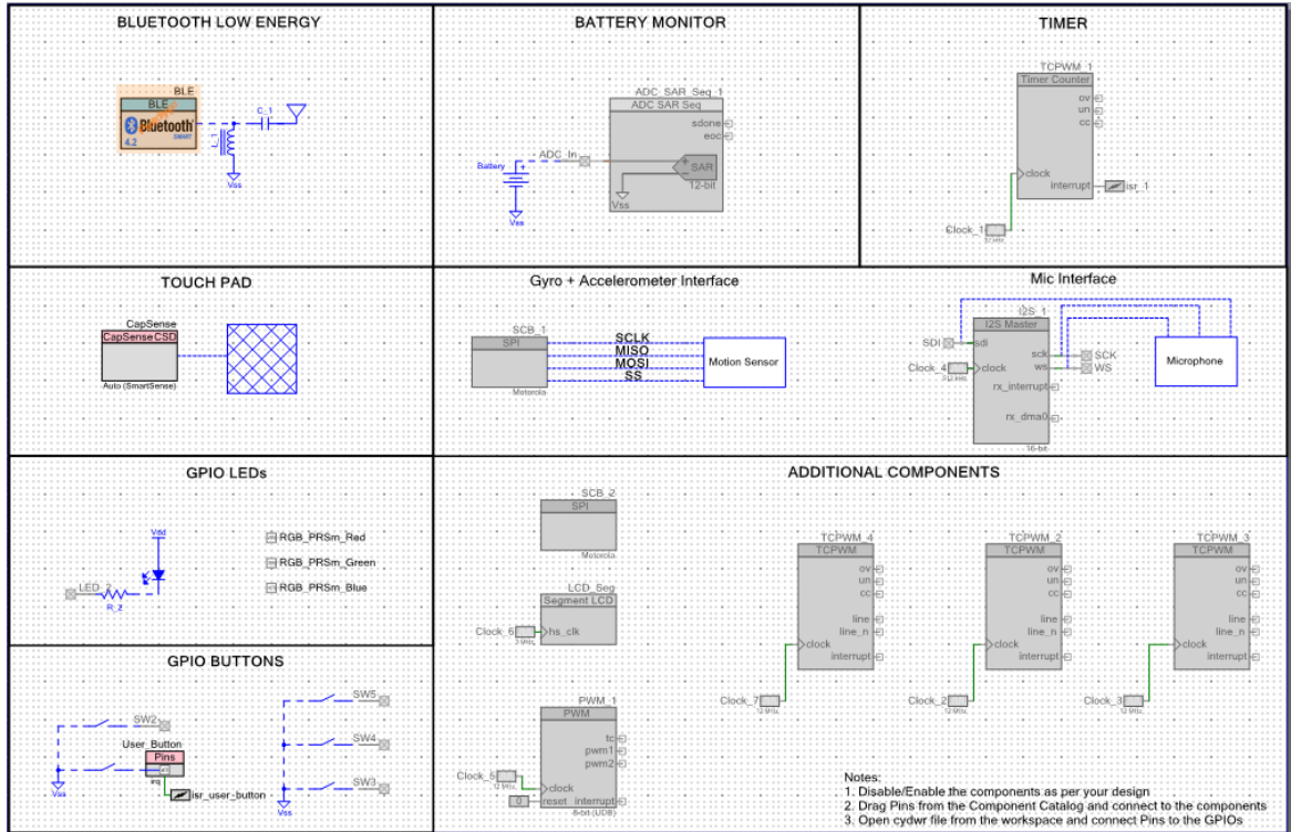
Figure 4-9. TopDesign for PProC_BLE_CapSense_Slider_LED Project
