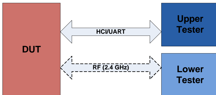
Figure 4-98. Direct Test Mode (DTM) Setup
