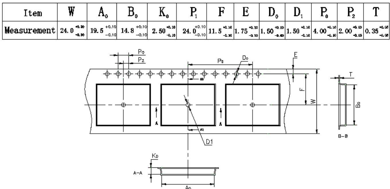
Figure 10. CYBLE-212019-00 Tape Dimensions
