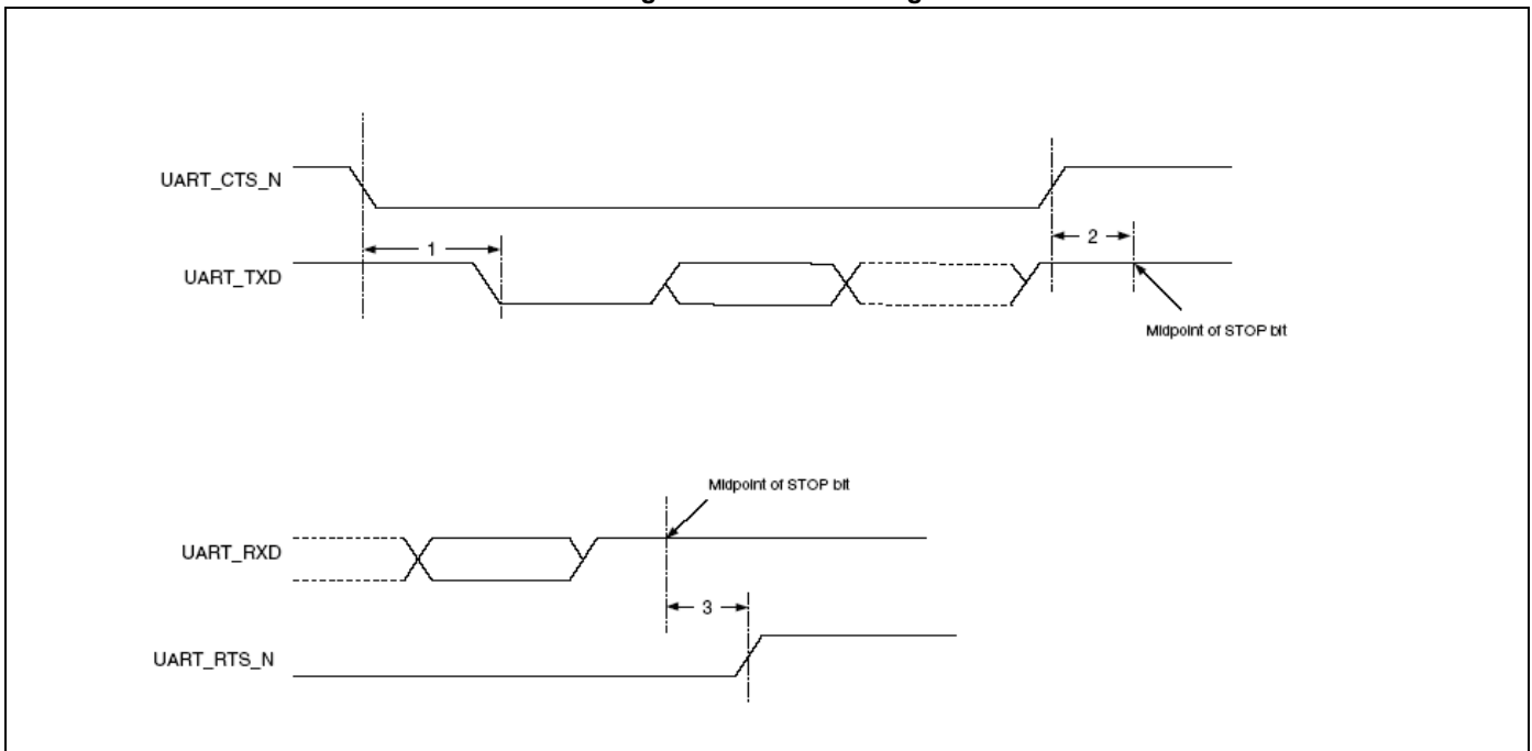
Figure 10. UART Timing
