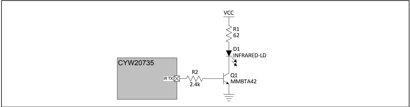
Figure 6. Infrared TX
