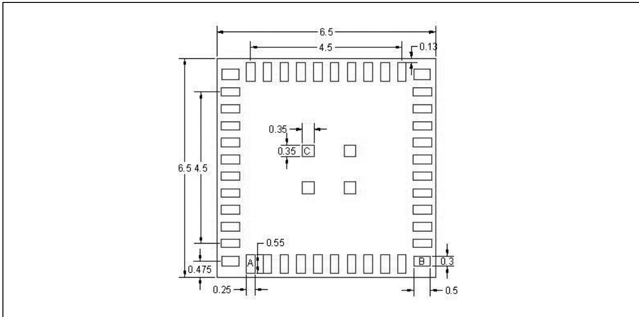
Figure 1-8. CYW20736E Stencil (Bottom View)
