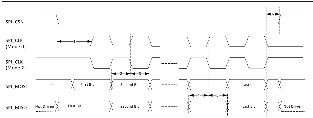
Figure 1-4. SPI Timing—Modes 0 and 2
