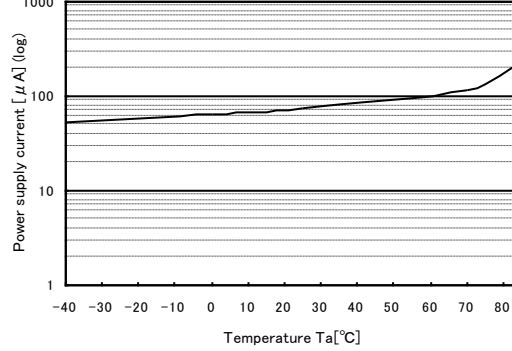
I_{OCT} timer mode(sub oscillation) temperature characteristics(semi-log) Vcc:5.5V, LVD is Off
