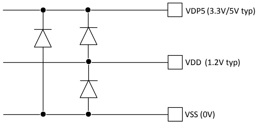
Figure 23. ESD Diodes between VDP5, VDD and VSS
