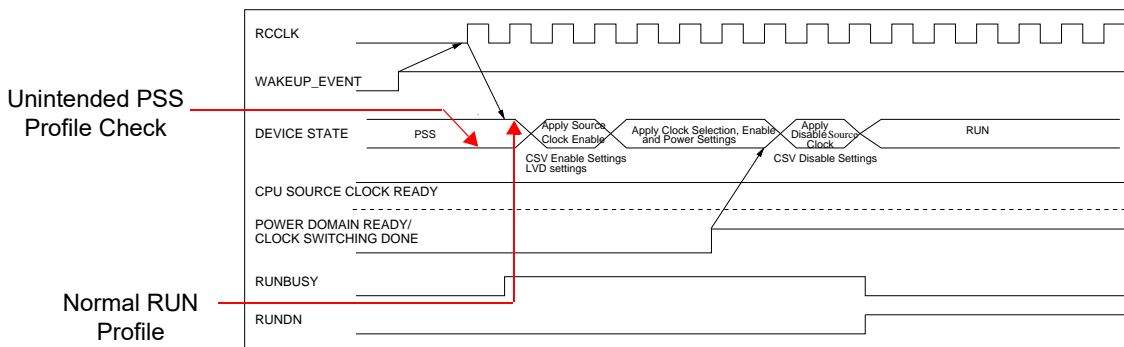
Figure 30. PSS to RUN State Switching
