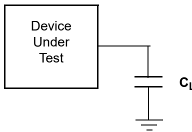
Figure 134. Test Setup
