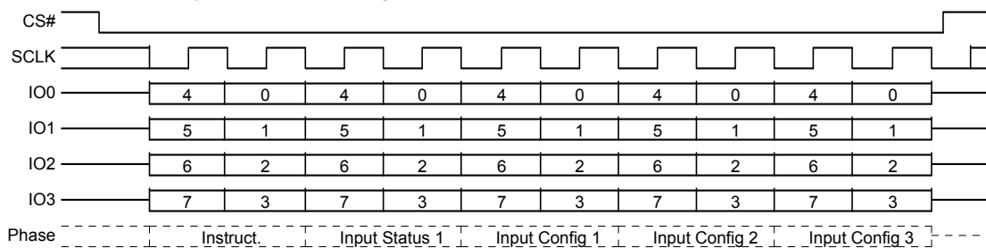
Figure 8.14 Write Register (WRR) Command Sequence QPI Mode
