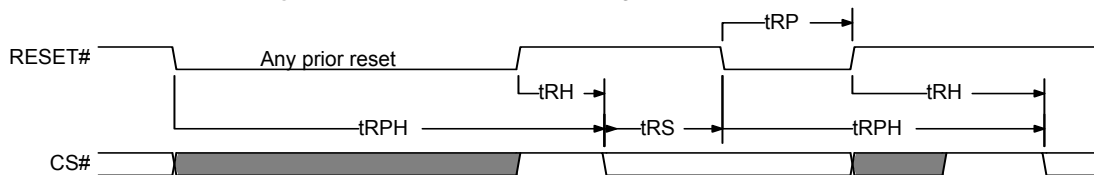
Figure 12.7 Hardware Reset using RESET# Input
