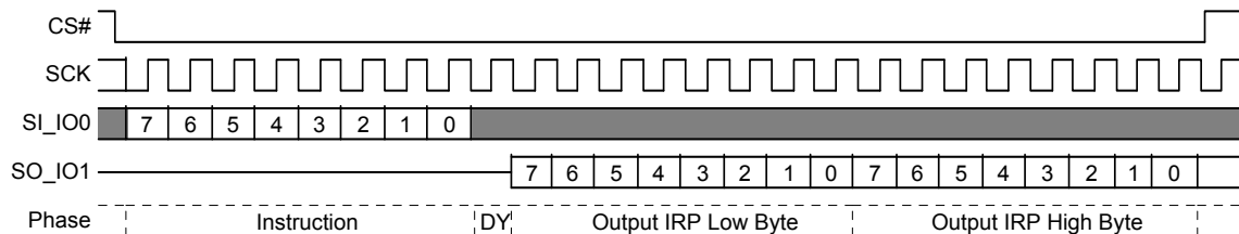
Figure 8.81 IRPRD Command Sequence
