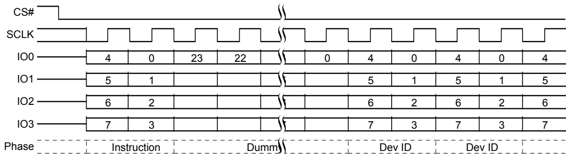
Figure 8.102 Read Identification (RES) QPI Mode Command
