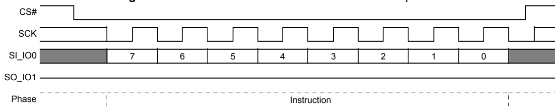
Figure 8.95 Software / Mode Bit Reset Command Sequence
