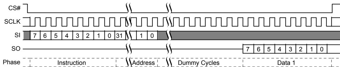
Figure 5.6 Single Bit Wide I/O Command with latency
