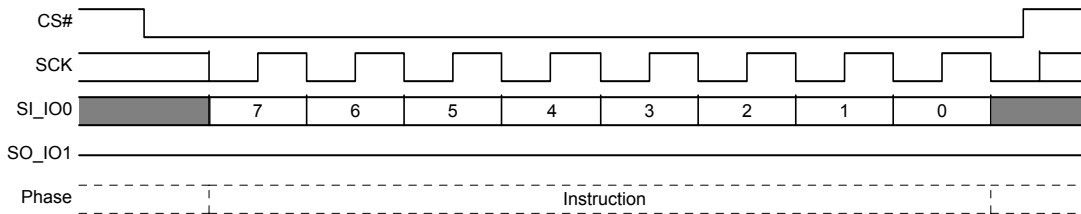
Figure 8.15 Write Enable (WREN) Command Sequence
