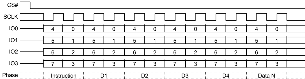
Figure 8.2 Read Identification (RDID) QPI Mode Command
