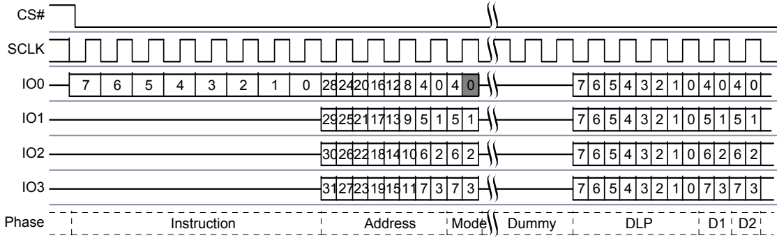
Figure 5.12 DDR Quad I/O Read Command
