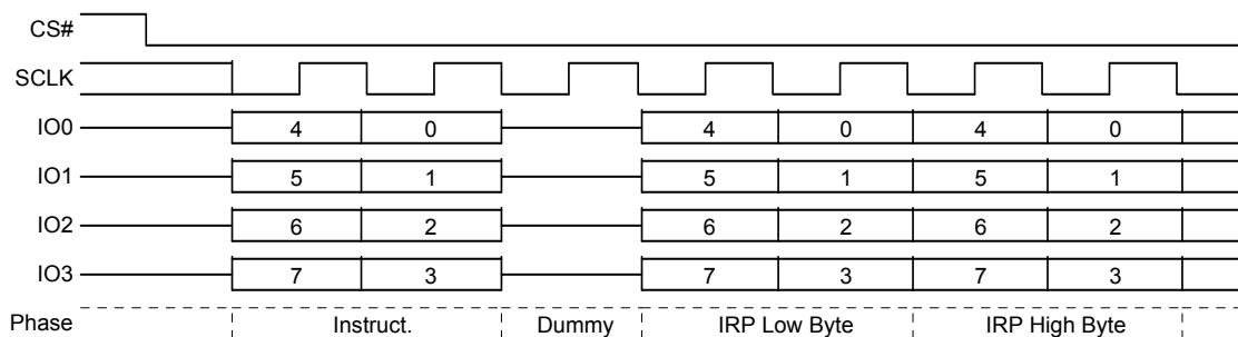
Figure 8.82 IRPRD Command Sequence – QPI Mode
