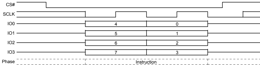
Figure 8.63 Program or Erase Suspend Command Sequence QPI mode
