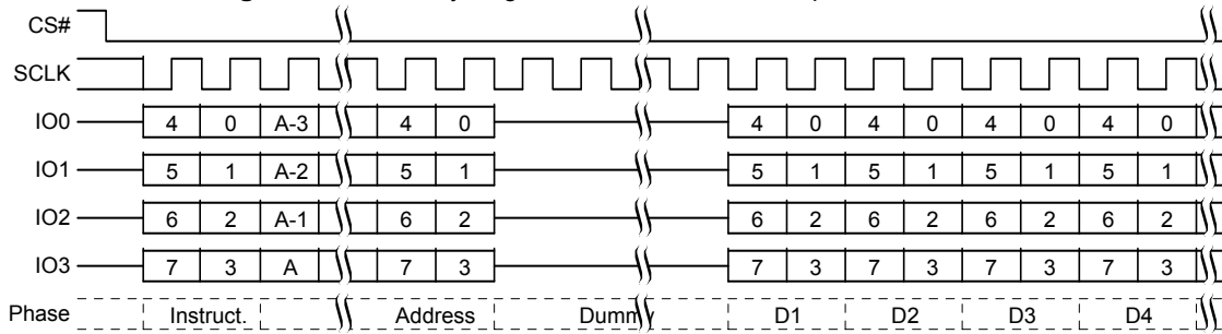
Figure 8.68 Security Regions Read Command Sequence QPI mode
