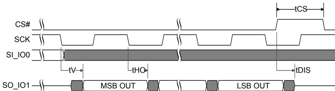
Figure 12.12 SPI Single Bit Output Timing
