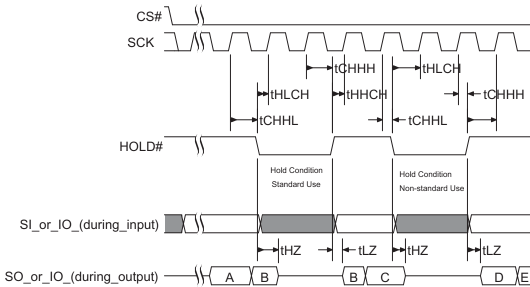
Figure 34. Hold Timing
