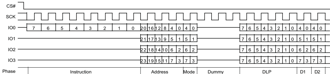
Figure 89 DDR Quad I/O Read Initial Access (3-Byte Address, EDh [ExtAdd=0], HPLC=11b)
