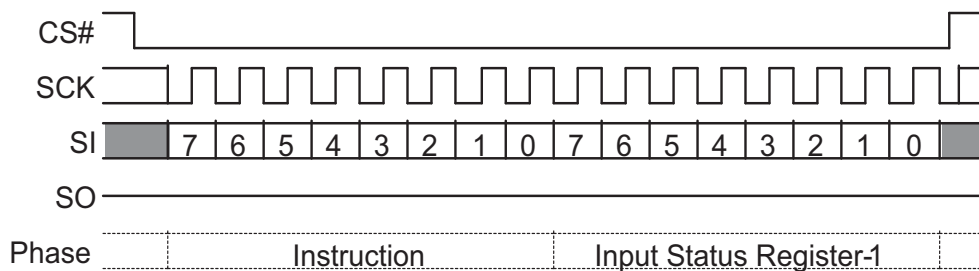
Figure 52 Write Registers (WRR 01h) Command Sequence – 8 data bits
