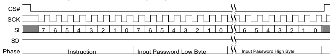
Figure 113 Password Program (PASSP E8h) Command Sequence
