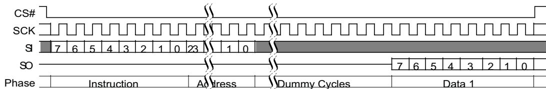
Figure 45 RSFDP Command Sequence
