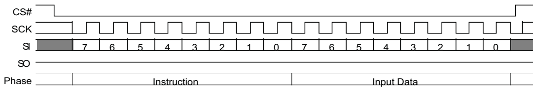
Figure 50 Bank Register Write (BRWR 17h) Command
