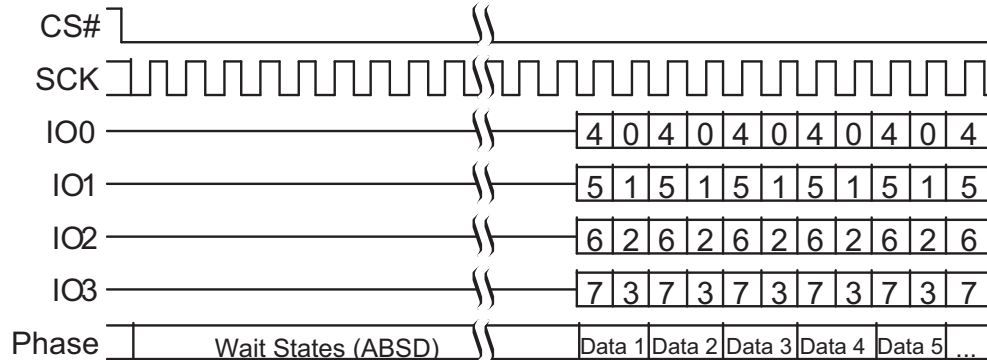
Figure 59 AutoBoot Sequence (CR1[1]=1)
