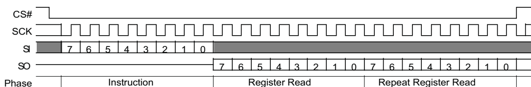
Figure 49 Read Bank Register (BRRD 16h) Command
