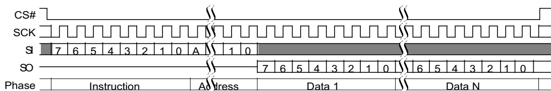
Figure 65 Read Command Sequence (READ 03h or 13h)
