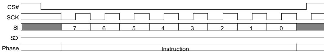
Figure 111 PPB Lock Bit Write (PLBWR A6h) Command Sequence
