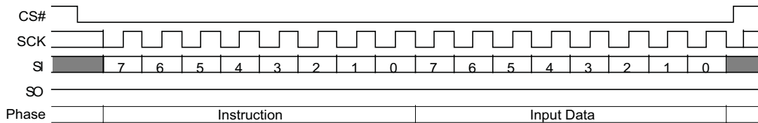
Figure 62 Program NVDLR (PNVDLR 43h) Command Sequence
