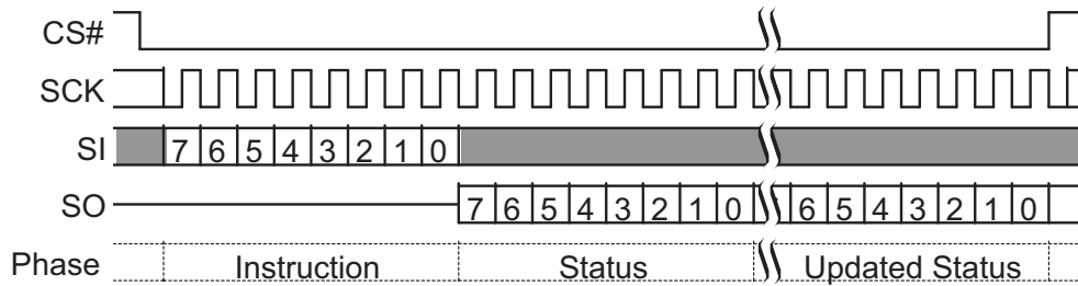
Figure 47 Read Status Register-2 (RDSR2 07h) Command Sequence
