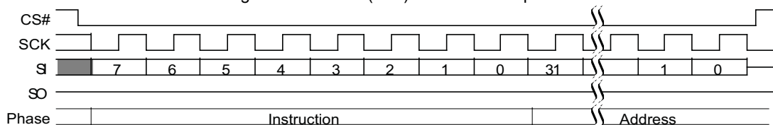
Figure 108 PPBP (E3h) Command Sequence
