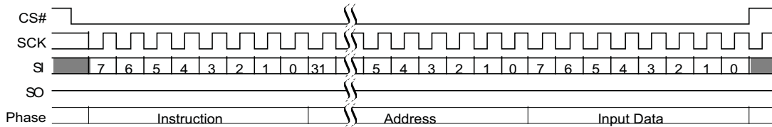
Figure 106 DYBWR (E1h) Command Sequence
