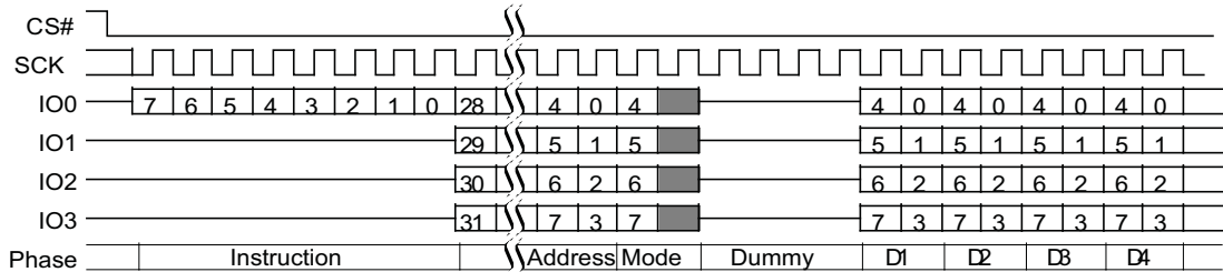
Figure 15 Quad I/O Command
