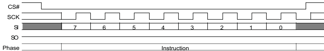
Figure 55 Write Disable (WRDI 04h) Command Sequence
