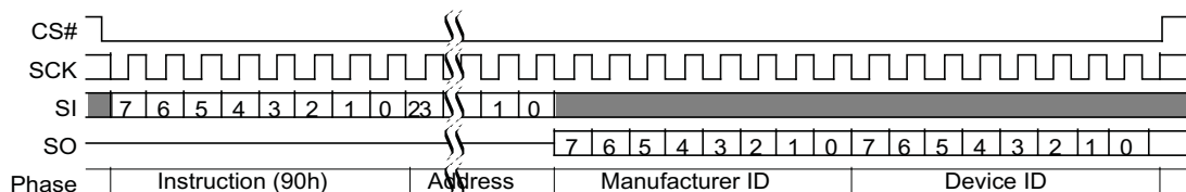
Figure 42 READ_ID (90h) Command Sequence
