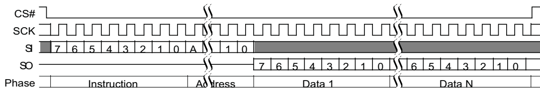
Figure 67 Fast Read Command (FAST_READ 0Bh or 0Ch) Sequence without Read Latency
