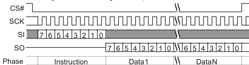
Figure 60 AutoBoot Register Read (ABRD 14h) Command
