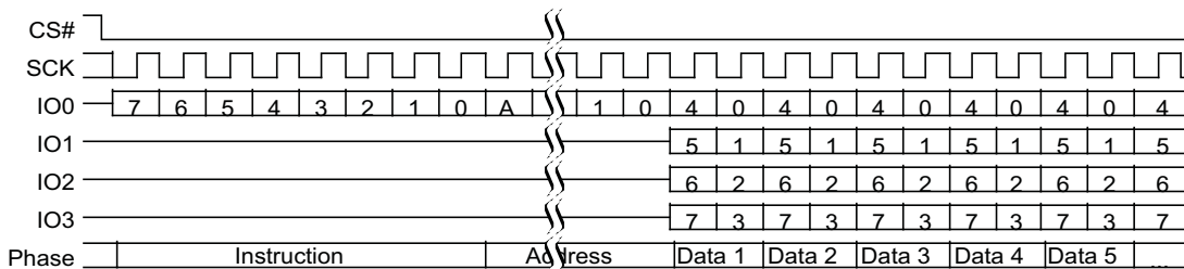
Figure 72 Quad Output Read (QOR 6Bh or 4QOR 6Ch) Command Sequence without Read Latency
