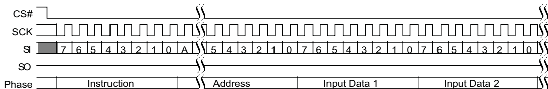
Figure 93 Page Program (PP 02h or 4PP 12h) Command Sequence
