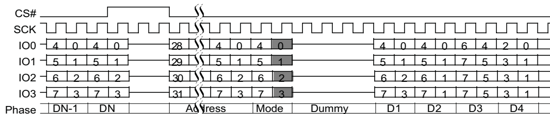
Figure 80 Continuous Quad I/O Read Command Sequence (4-Byte Address), LC=00b
