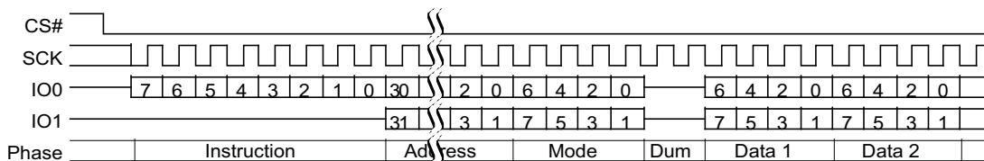
Figure 75 Dual I/O Read Command Sequence (4-Byte Address, BCh or BBh [ExtAdd=1], EHPLC=10b)
