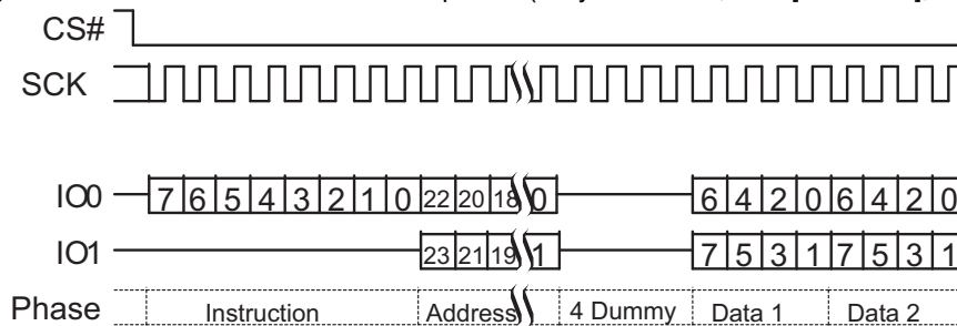
Figure 73 Dual I/O Read Command Sequence (3-Byte Address, BBh [ExtAdd=0], HPLC=00b)
