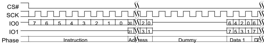
Figure 88 DDR Dual I/O Read (4-Byte Address, BEh or BDh [ExtAdd=1], HPLC=00b)
