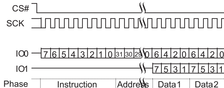
Figure 70 Dual Output Read Command Sequence (4-Byte Address, 3Ch or 3Bh [ExtAdd=1, LC=11b])
