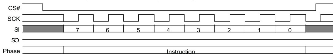
Figure 109 PPB Erase (PPBE E4h) Command Sequence
