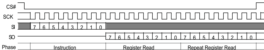
Figure 48 Read Configuration Register (RDCR 35h) Command Sequence
