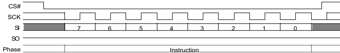
Figure 56 Clear Status Register (CLSR 30h) Command Sequence
