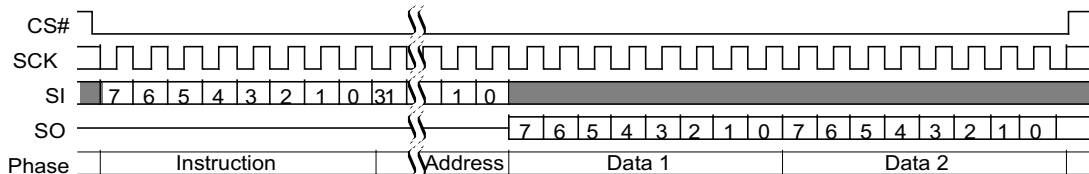
Figure 10 Single Bit Wide I/O Command without Latency
