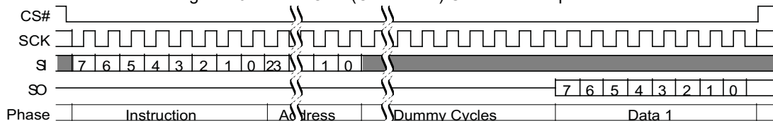
Figure 102 Read OTP (OTPR 4Bh) Command Sequence
