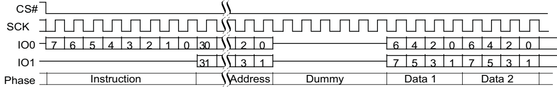
Figure 14 Dual I/O Command
