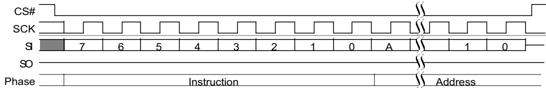
Figure 97 Sector Erase (SE D8h or 4SE DCh) Command Sequence
