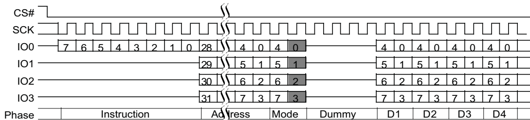
Figure 79 Quad I/O Read Command Sequence(4-Byte Address, ECh or EBh [ExtAdd=1], LC=00b)
