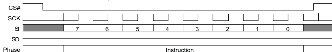
Figure 98 Bulk Erase Command Sequence
