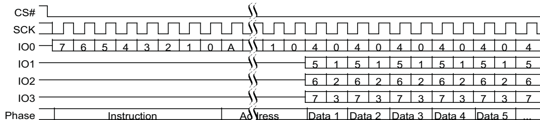
Figure 94 Quad 512-byte Page Program Command Sequence
