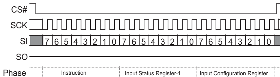
Figure 53 Write Registers (WRR 01h) Command Sequence – 16 data bits
