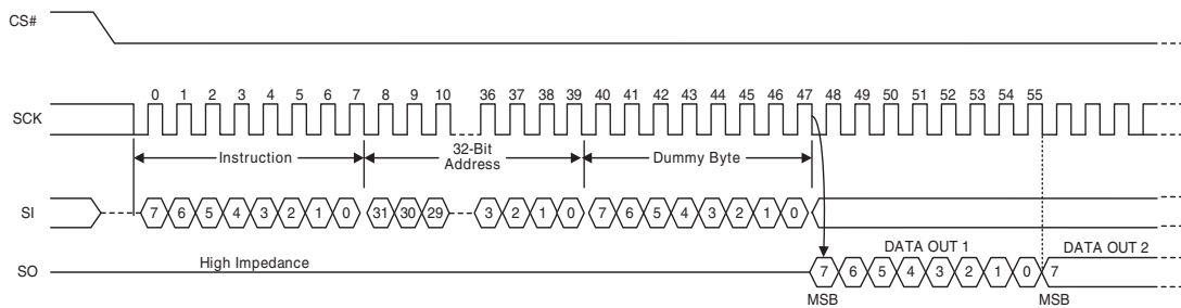
Figure 57 ECC Status Register Read Command Sequence
