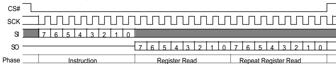
Figure 110 PPB Lock Register Read Command Sequence
