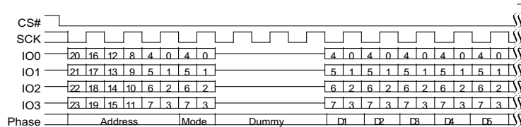
Figure 90 Continuous DDR Quad I/O Read Subsequent Access (3-Byte Address, HPLC=11b)
