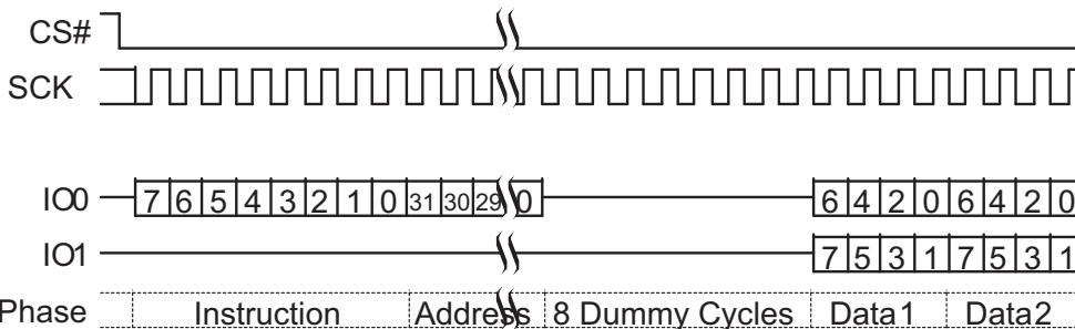
Figure 69 Dual Output Read Command Sequence (4-Byte Address, 3Ch or 3Bh [ExtAdd=1, LC=10b])
