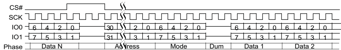
Figure 76 Continuous Dual I/O Read Command Sequence (4-Byte Address, BCh or BBh [ExtAdd=1], EHPLC=10b)
