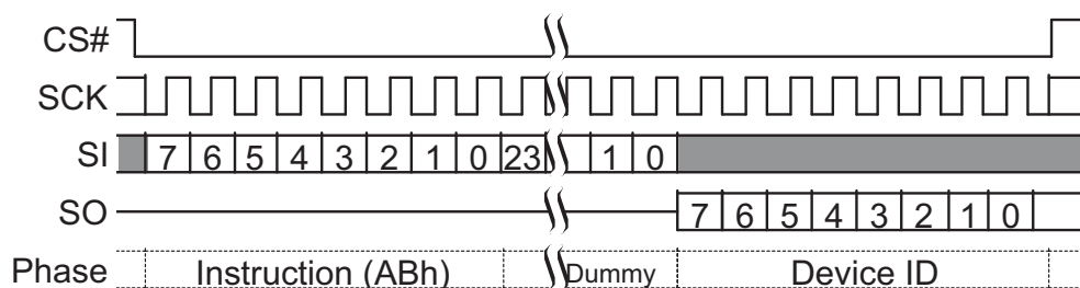
Figure 44 Read Electronic Signature (RES ABh) Command Sequence
