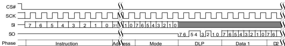
Figure 83 DDR Fast Read Initial Access (4-Byte Address, 0Eh or 0Dh [ExtAdd=1], EHPLC=01b)
