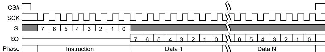
Figure 64 DLP Read (DLPRD 41h) Command Sequence
