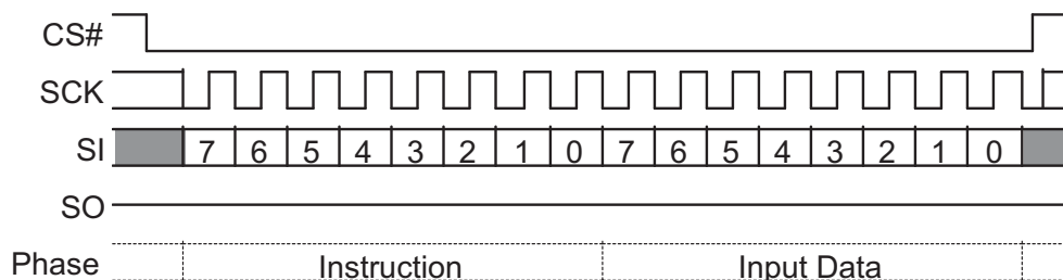
Figure 63 Write VDLR (WVDLR 4Ah) Command Sequence
