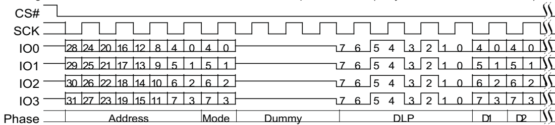
Figure 92 Continuous DDR Quad I/O Read Subsequent Access (4-Byte Address, EHPLC=01b)
