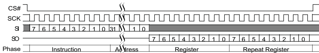
Figure 107 PPBRD (E2h) Command Sequence
