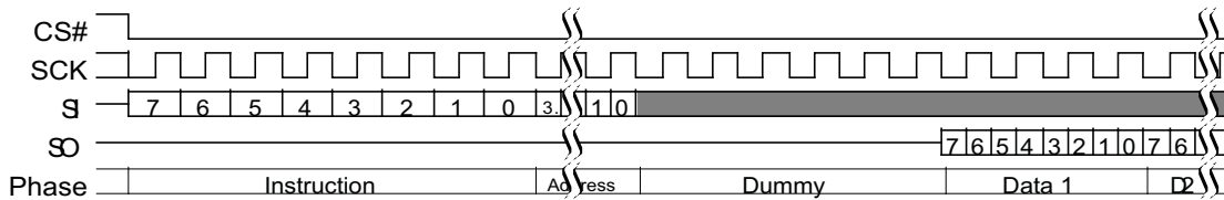
Figure 85 DDR Fast Read Subsequent Access (4-Byte Address, HPLC=01b)
