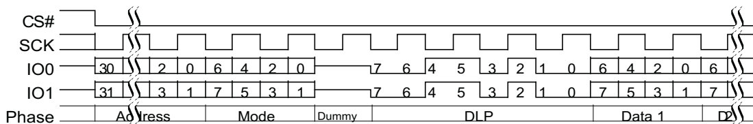
Figure 87 Continuous DDR Dual I/O Read Subsequent Access (4-Byte Address, EHPLC= 01b)
