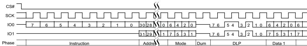
Figure 86 DDR Dual I/O Read Initial Access (4-Byte Address, BEh or BDh [ExtAdd=1], EHPLC= 01b)
