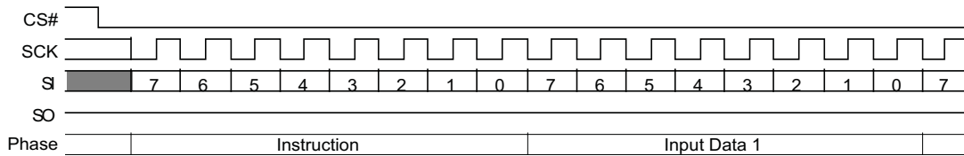
Figure 61 AutoBoot Register Write (ABWR) Command
