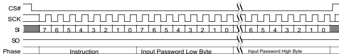
Figure 114 Password Unlock (PASSU E9h) Command Sequence
