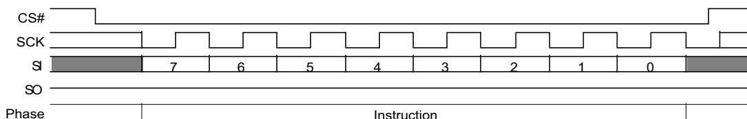
Figure 51 BRAC (B9h) Command Sequence
