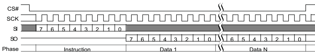
Figure 112 Password Read (PASSRD E7h) Command Sequence
