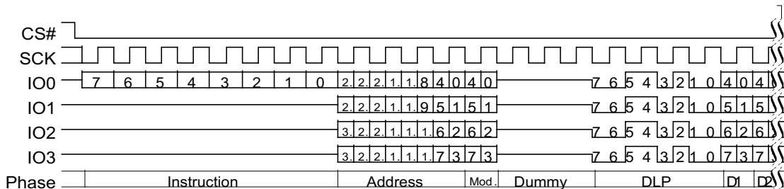
Figure 91 DDR Quad I/O Read Initial Access (4-Byte Address, EEh or EDh [ExtAdd=1], EHPLC=01b)
