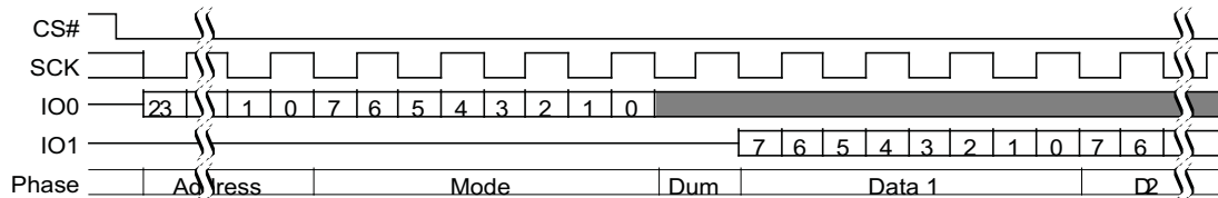
Figure 82 Continuous DDR Fast Read Subsequent Access (3-Byte Address [ExtAdd=0, EHPLC=11b])
