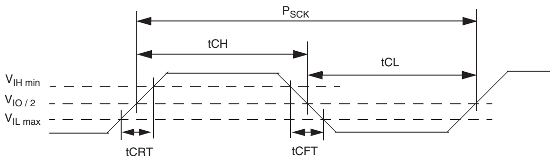
Figure 30 Clock Timing
