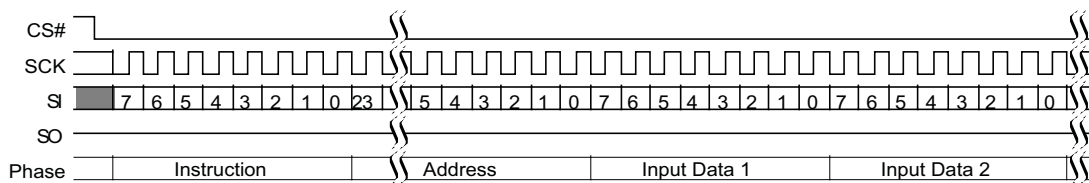
Figure 101 Page Program (OTPP 42h) Command Sequence
