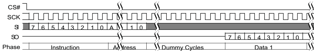
Figure 66 Fast Read (FAST_READ 0Bh or 0Ch) Command Sequence with Read Latency
