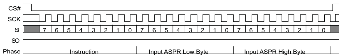
Figure 104 ASPP (2Fh) Command
