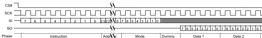
Figure 81 DDR Fast Read Initial Access (3-Byte Address, 0Dh [ExtAdd=0, EHPLC=11b])
