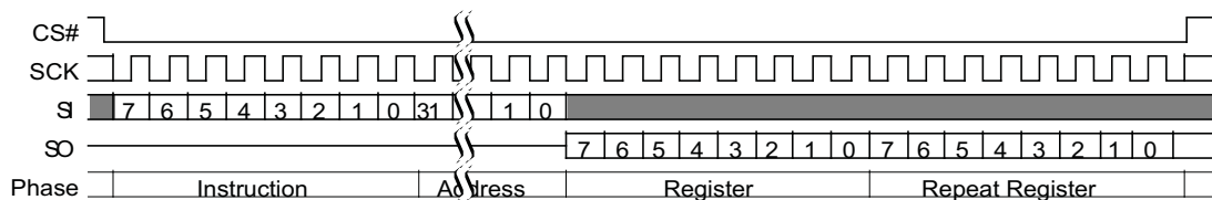
Figure 105 DYBRD Command Sequence
