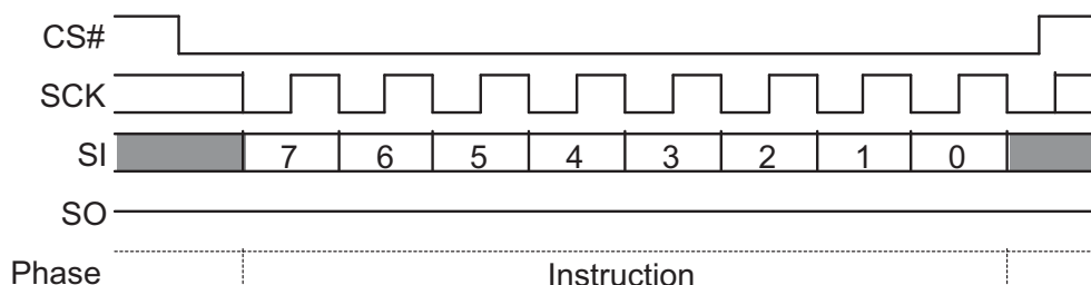
Figure 54 Write Enable (WREN 06h) Command Sequence
