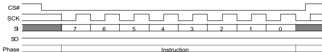
Figure 115 Software Reset (RESET F0h) Command Sequence
