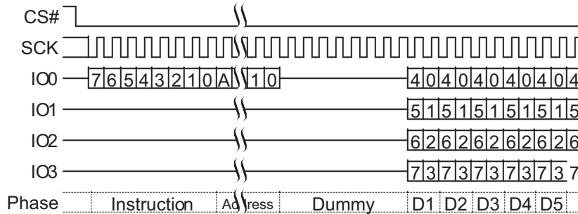
Figure 71 Quad Output Read (QOR 6Bh or 4QOR 6Ch) Command Sequence with Read Latency
