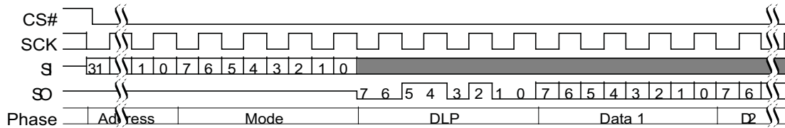
Figure 84 Continuous DDR Fast Read Subsequent Access (4-Byte Address [ExtAdd=1], EHPLC=01b)
