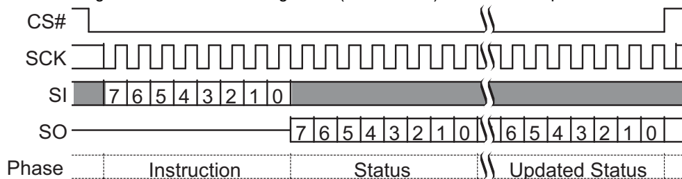
Figure 46 Read Status Register-1 (RDSR1 05h) Command Sequence
