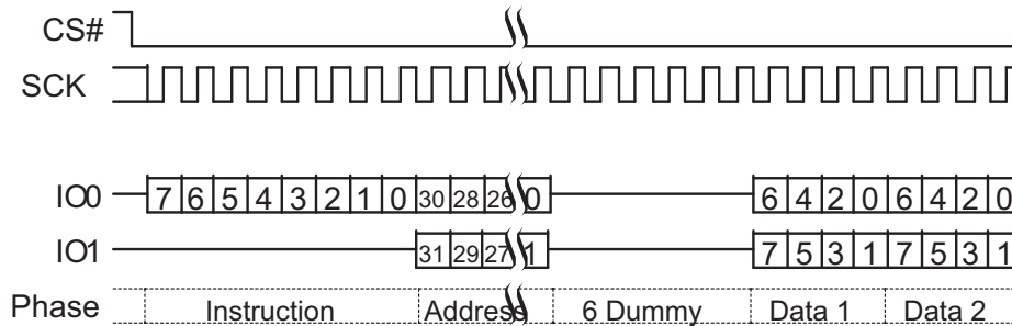
Figure 74 Dual I/O Read Command Sequence (4-Byte Address, BBh [ExtAdd=1], HPLC=10b)
