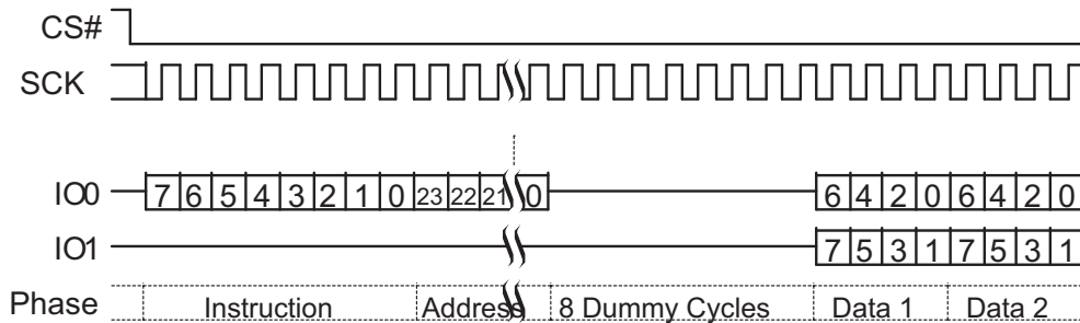
Figure 68 Dual Output Read Command Sequence (3-Byte Address, 3Bh [ExtAdd=0], LC=10b)
