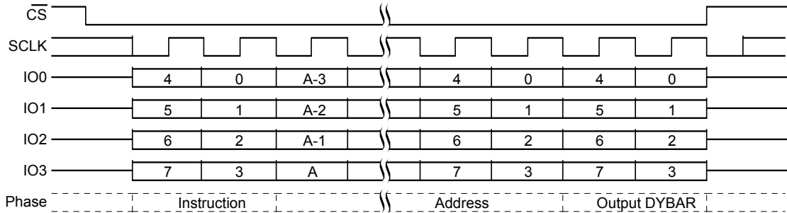
Figure 11.63 DYBRD QPI Mode Command Sequence
