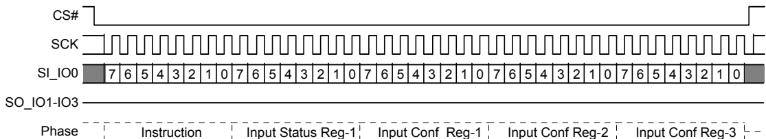
Figure 11.13 Write Register (WRR) Command Sequence
