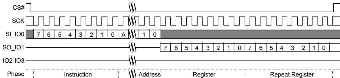
Figure 11.62 DYBRD Command Sequence
