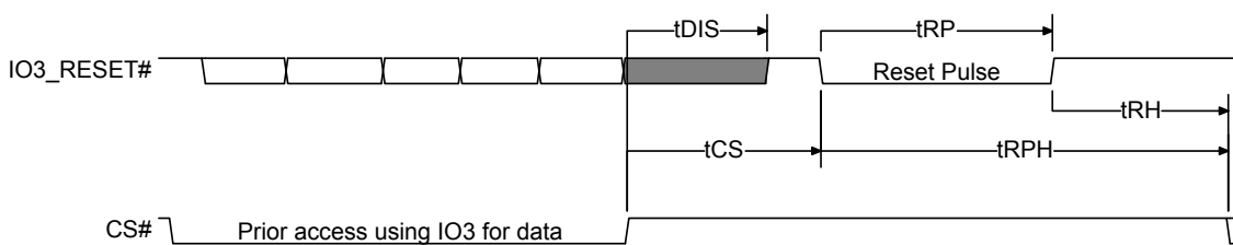
Figure 6.9 Hardware Reset when Quad or QPI Mode and IO3_RESET# are Enabled
