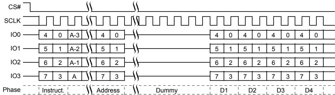
Figure 11.6 RSFDP QPI Mode Command Sequence
