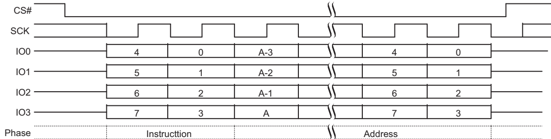
Figure 89. Parameter Sector Erase (P4E 20h or 4P4E 21h) QPI Mode Command Sequence [67]
