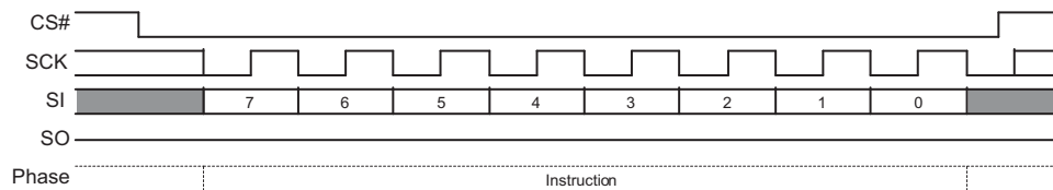
Figure 7. Single Bit Wide Input Command
