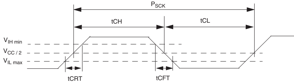
Figure 28. Clock Timing
