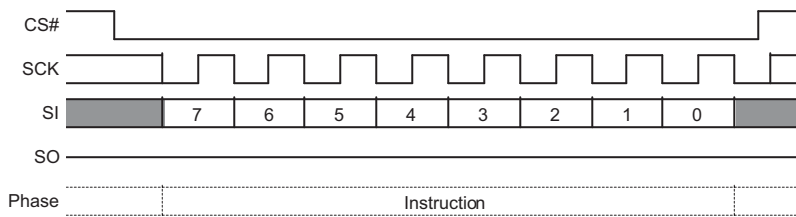
Figure 94. Erase or Program Suspend Command Sequence
