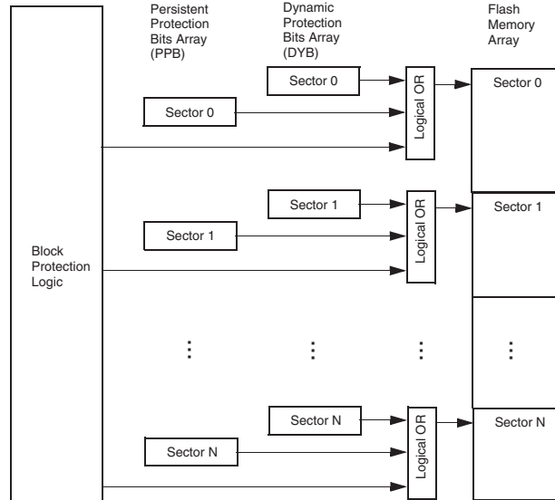
Figure 44. Advanced Sector Protection Overview
