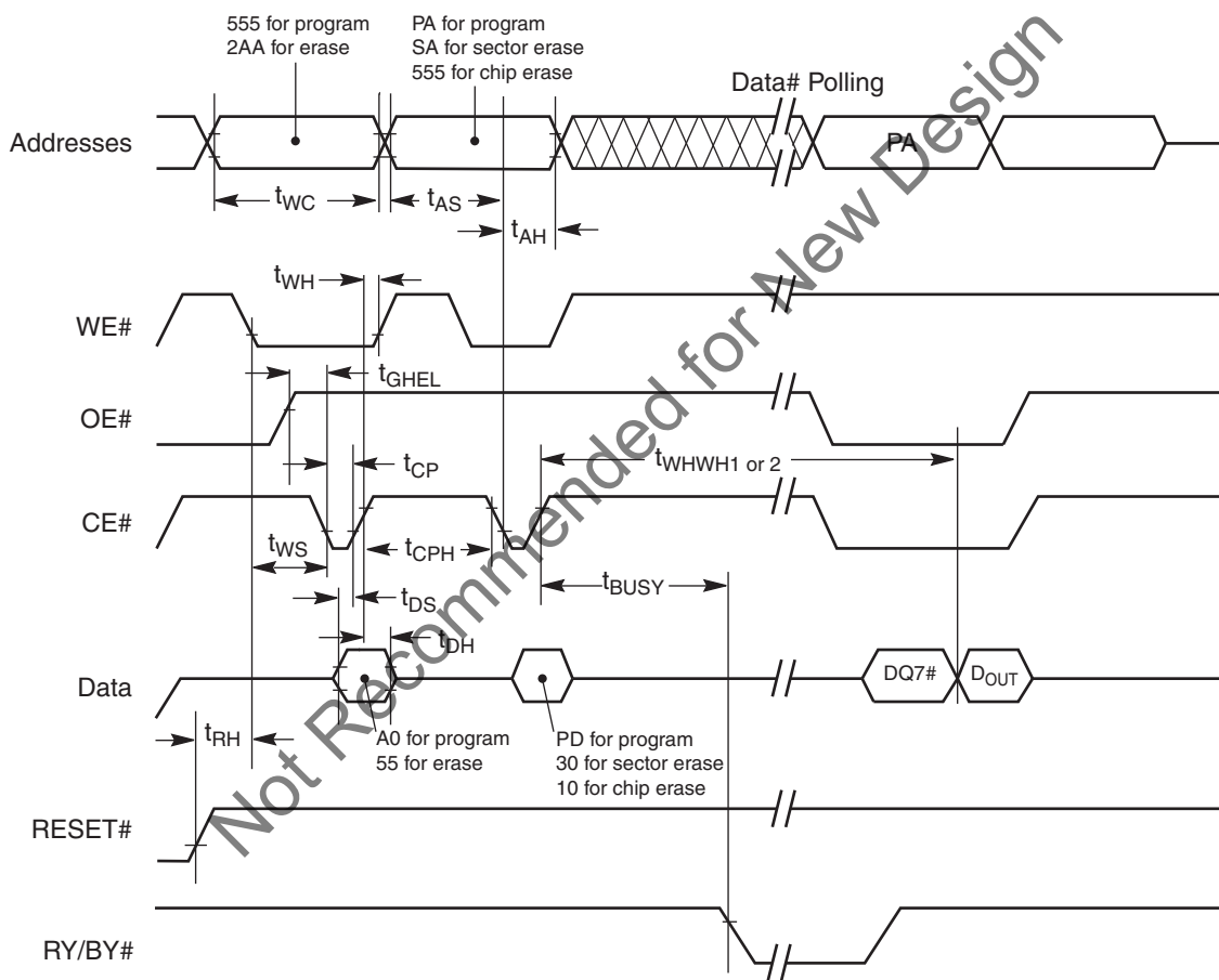
Figure 18.1 Alternate CE# Controlled Write Operation Timings
