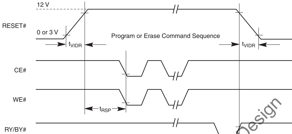
Figure 18.2 Accelerated Program Timing Diagram
