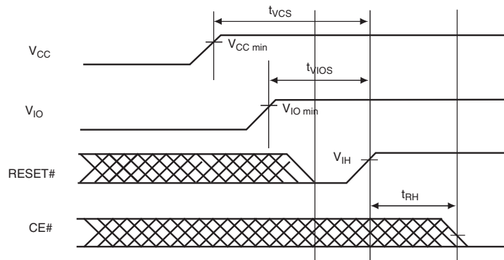
Figure 9. V CC Power-up Diagram.
