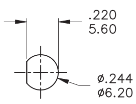
PANEL MOUNTING
