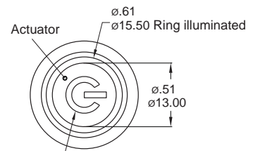
E1 Ring (Moveable)+Power logo
