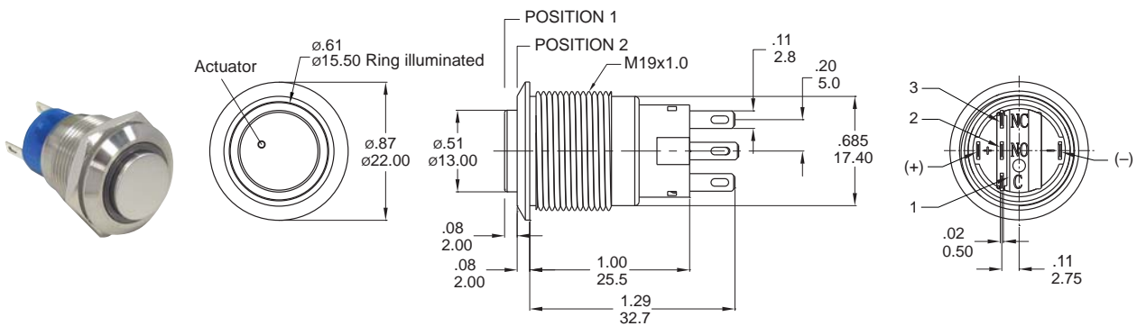
Part No. Shown : MPB19-A0H1□R-□□-JQ
