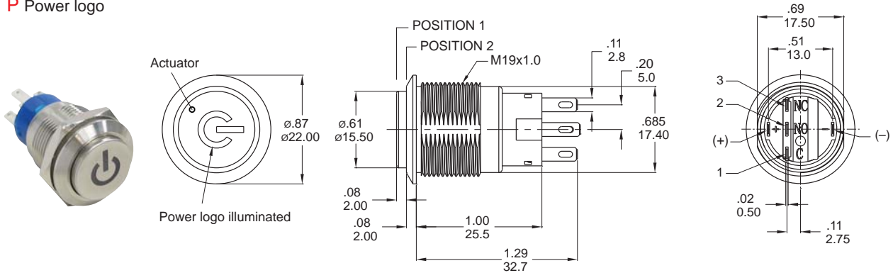
Part No. Shown : MPB19-D0H1□P-□□-JQ
